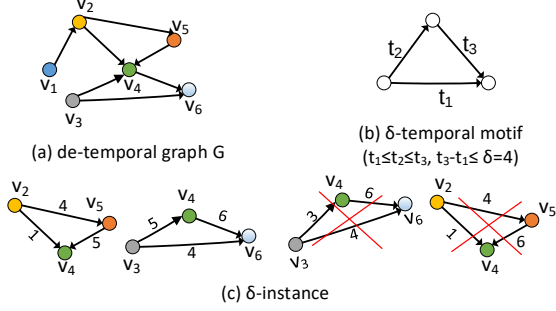
Figure 2: The latter two of (c) are not \delta -instances because they respectively violate conditions (i) and (ii) in Definition 2.
